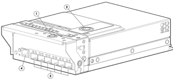
Figure 1 6SFP Uplink Module Components
