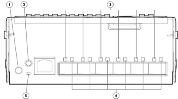
Figure 2 6SFP Uplink Module buttons and LED
