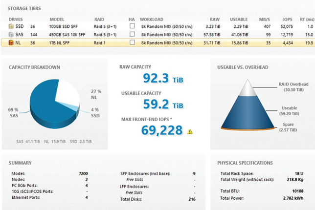
Figure 1: System configuration and capacity details
