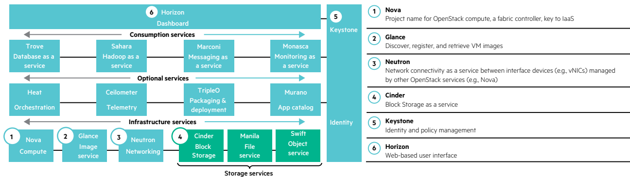
Figure 1: OpenStack architecture basics
