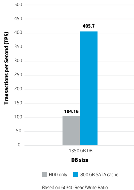
Figure 1. OLTP performance with SmartCache
