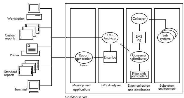
Figure 1: EMS Analyzer Architecture
