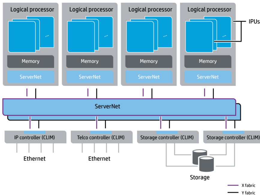
Figure 2. An HP NonStop i System Architecture
