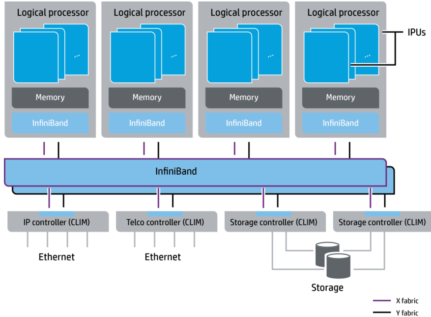
Figure 2. An HP NonStop i System Architecture
