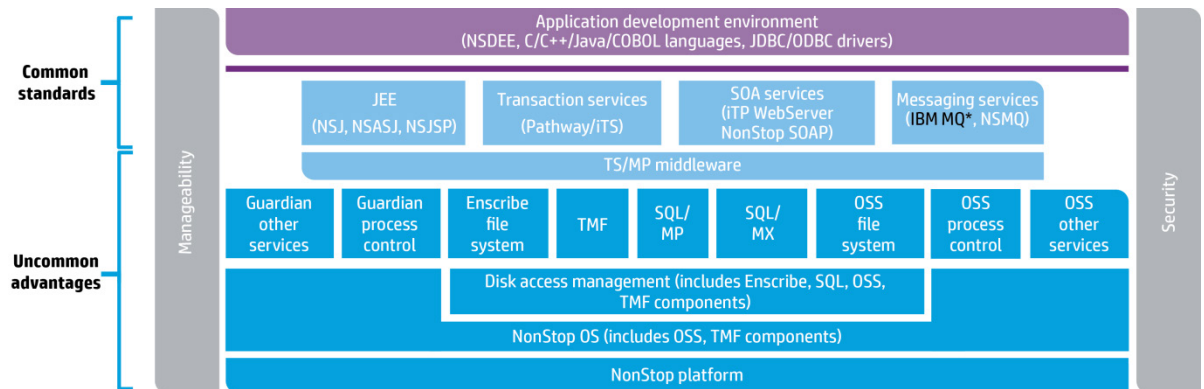
Figure 5. NonStop OS supports industry-standard APIs used by modern business applications
